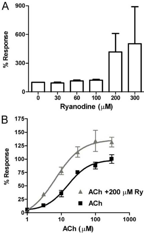
FIG. 2. Ryanodine increases the sensitivity of the \alpha 9\alpha 10 nAChR for ACh. A Mean and standard error of the percent change in response to 10 \mu\text{M} ACh (at -70 mV, internal BAPTA buffering) for different concentrations of ryanodine (30, 60, 100, and 200 \mu\text{M} , n=3-9 per concentration). B Concentration-response curves to ACh in the absence and presence of 200 \mu\text{M} ryanodine ( n=3-7 per concentration). Ryanodine increased the apparent affinity of the recombinant \alpha 9\alpha 10 nAChR for ACh and also the amplitude of responses to saturating concentrations of this agonist. V_{\text{hold}}=-70 mV.
