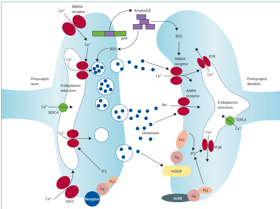
Figure 4: Mechanisms of synaptic dysfunction in ageing and Alzheimer's disease APP is axonally transported and so is present in high concentrations in presynaptic terminals. In properly functioning synapses, APP is proteolytically cleaved in the middle of the amyloid \beta sequence by \alpha secretase, thereby preventing the production of amyloid \beta . During normal ageing, and more so in Alzheimer's disease, APP is cleaved at the N-terminal and C-terminal of amyloid \beta by \beta secretase and \gamma secretase, respectively, resulting in the production and self-aggregation of amyloid \beta . Aggregation of amyloid \beta on the membrane generates ROS, which results in membrane lipid peroxidation. This in turn impairs the function of membrane ion-motive ATPases, thereby promoting membrane depolarisation and calcium influx through NMDA receptor channels and voltage-dependent calcium channels. Sustained increases in cytoplasmic calcium concentrations promote depletion of presynaptic glutamate stores, resulting in impaired synaptic transmission and damage to axons and dendrites. Additionally, disrupted mitochondrial function caused by ageing, oxidative stress, and amyloid \beta results in energy depletion in neurons, which exacerbates synaptic dysfunction and degeneration of neurons. Dysregulation of endoplasmic reticulum function, which results in depletion of endoplasmic reticulum calcium stores and accumulation of misfolded proteins further contributes to the death of neurons in Alzheimer's disease. APP=amyloid precursor protein. ROS=reactive oxygen species. SERCA=sarco/endoplasmic reticulum \text{Ca}^{2+} -ATPase. RyR=ryanodine receptor. IP3R=inositol trisphosphate receptor. PLC=phospholipase C. mGluR=metabotropic glutamate receptor. AchR=acetylcholine receptor. VDCC=voltage-dependent calcium channel.
